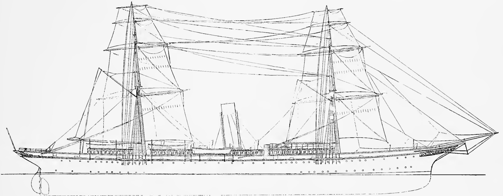
W. K. VANDERBILT'S TWIN-SCREW STEAM YACHT VALIANT.—Built by Laird Bros., Birkenhead, England.
